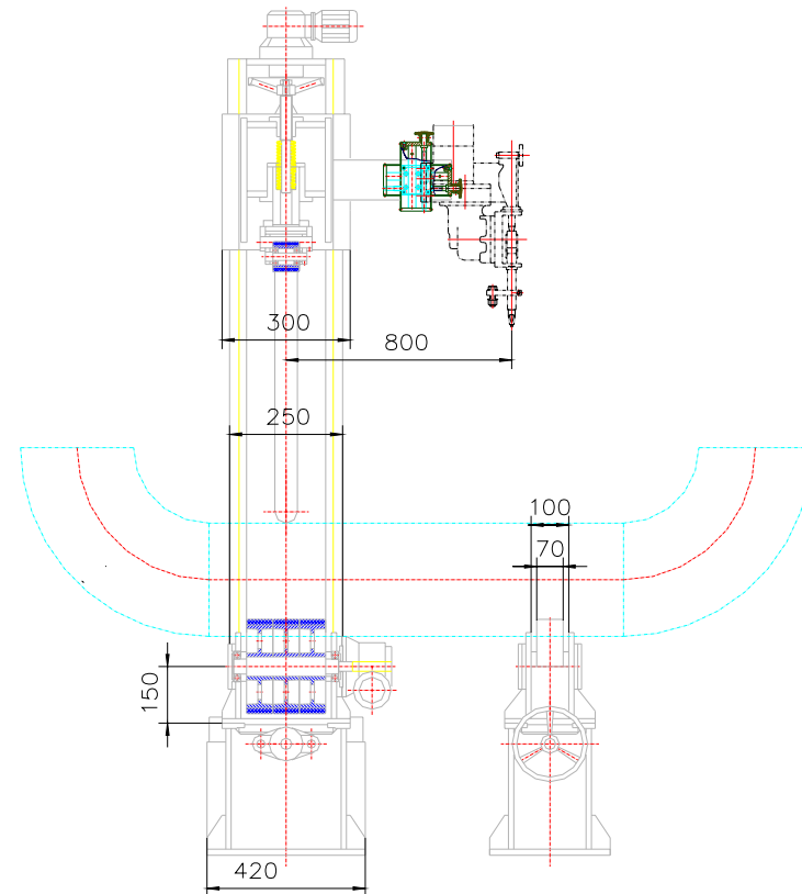
PIPE ROTATOR PR 5 CUSTOM BUILT W/ WELDING HEAD
