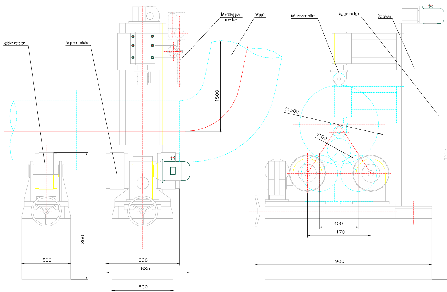
PIPE ROTATOR PR 25
