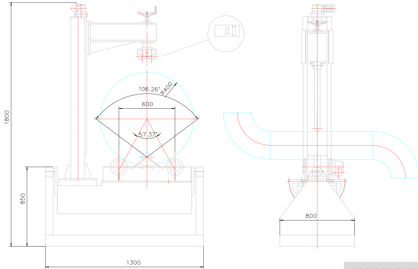
PIPE POSITIONER PP-3
